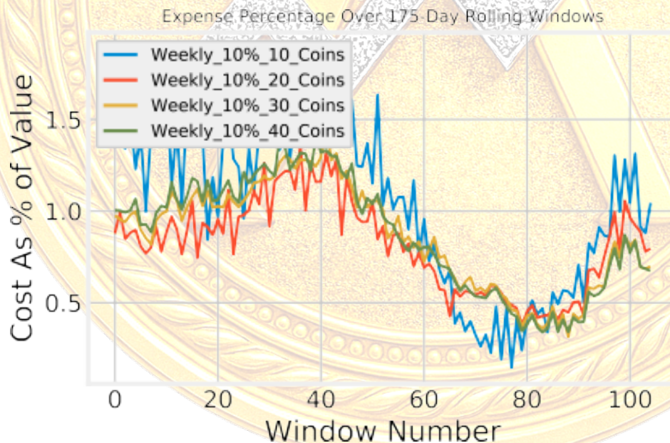
Fig. 7. Expenses for Different Number of Coins
