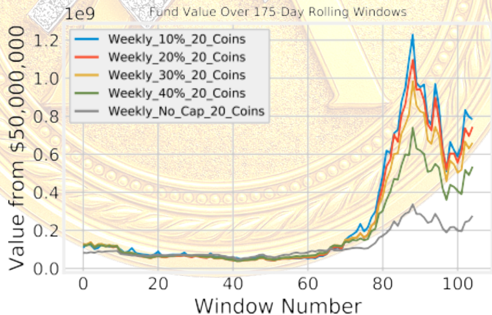
Fig. 8. Portfolio Performance for Different Market Caps
